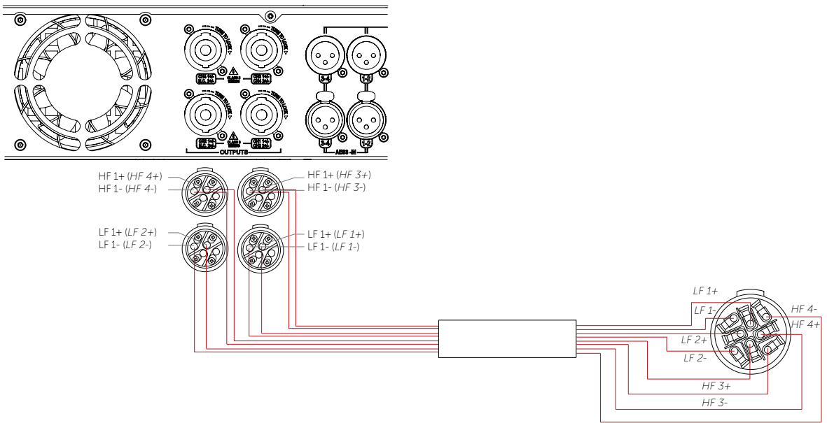
Figure 4.4: Bias Q3
